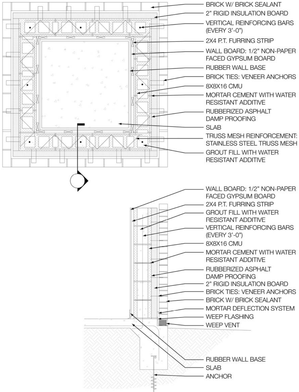
Fig. B.2. DIAGRAM: Detailed drawings, test pod B: cavity wall.
